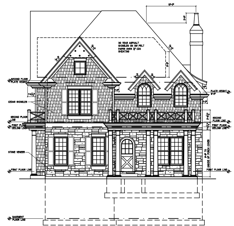
EAST SIDE ELEVATION
