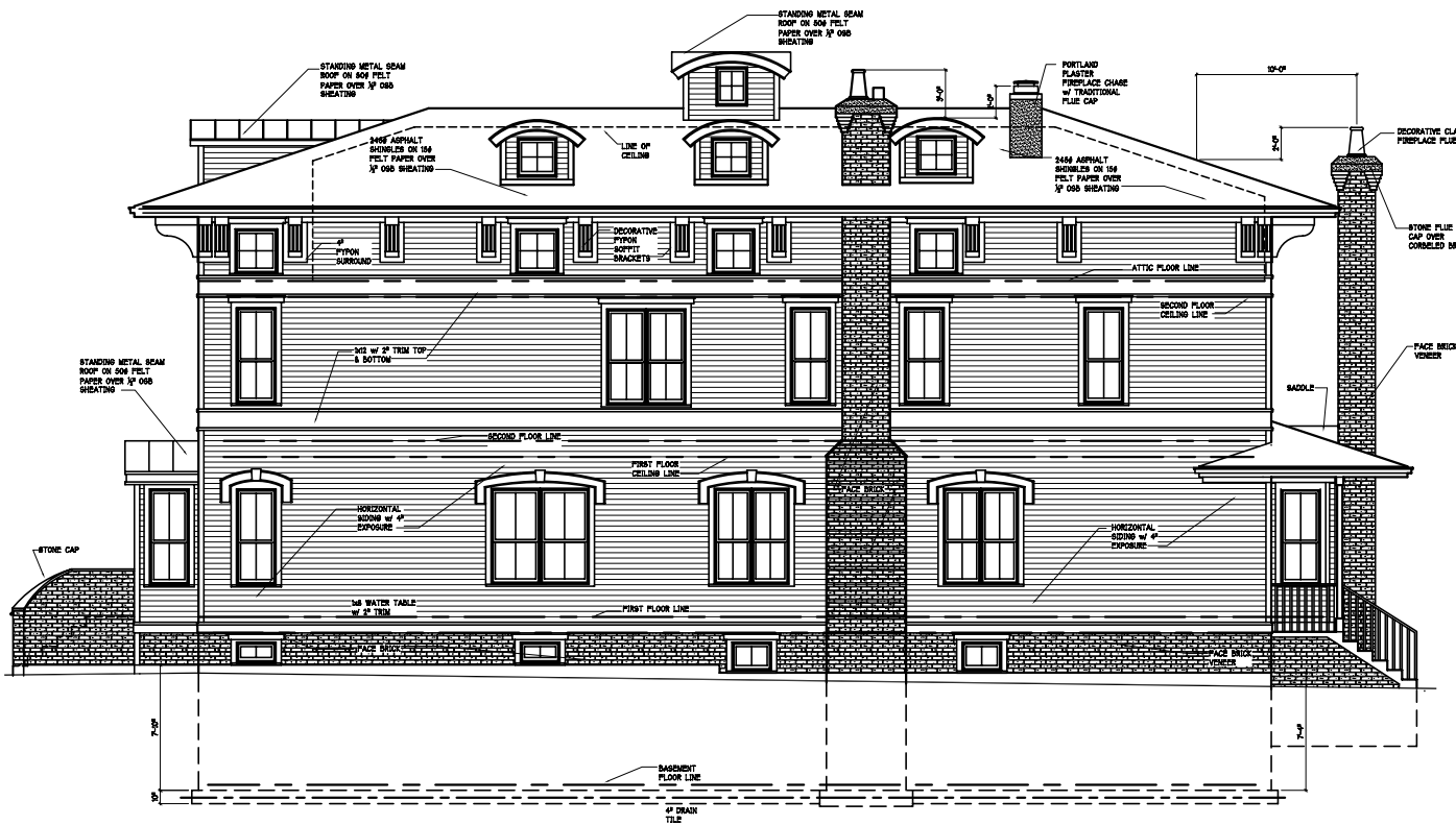
NORTH ELEVATION
